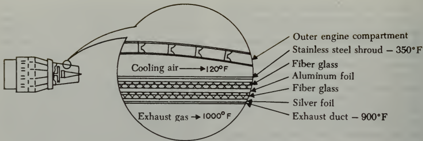
FIGURE 6-49. Typical engine insulation blanket.
